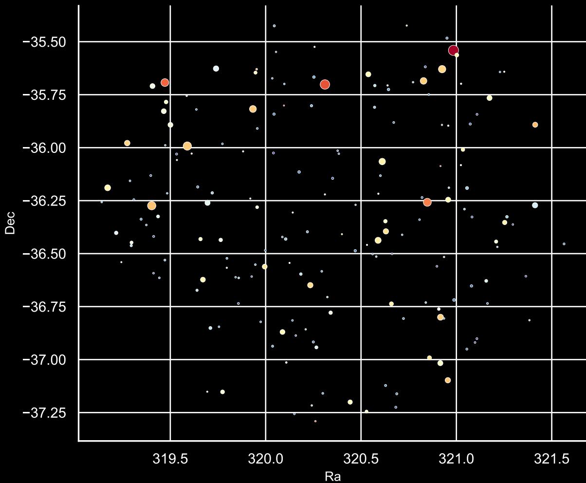
Field [43] Ra [320.31] Dec [-36.32] Stars: 180
