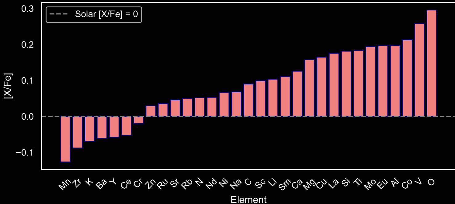
Abundance Pattern for GALAH Red Giants: Star Field [43] (N=53)
