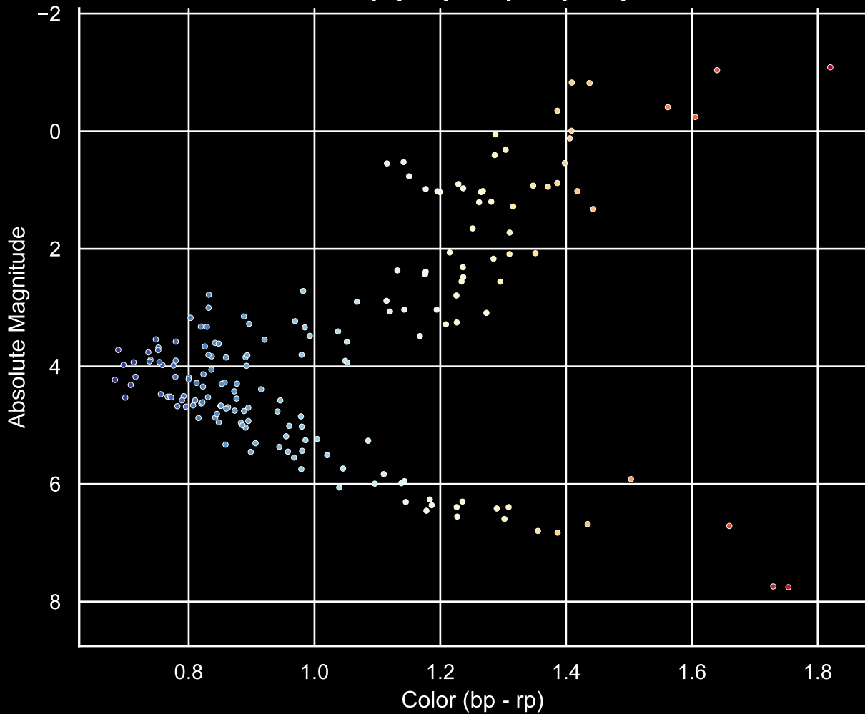
GALAH Hertzprung-Russel Diagram Field [43] Ra [320.31] Dec [-36.32]
