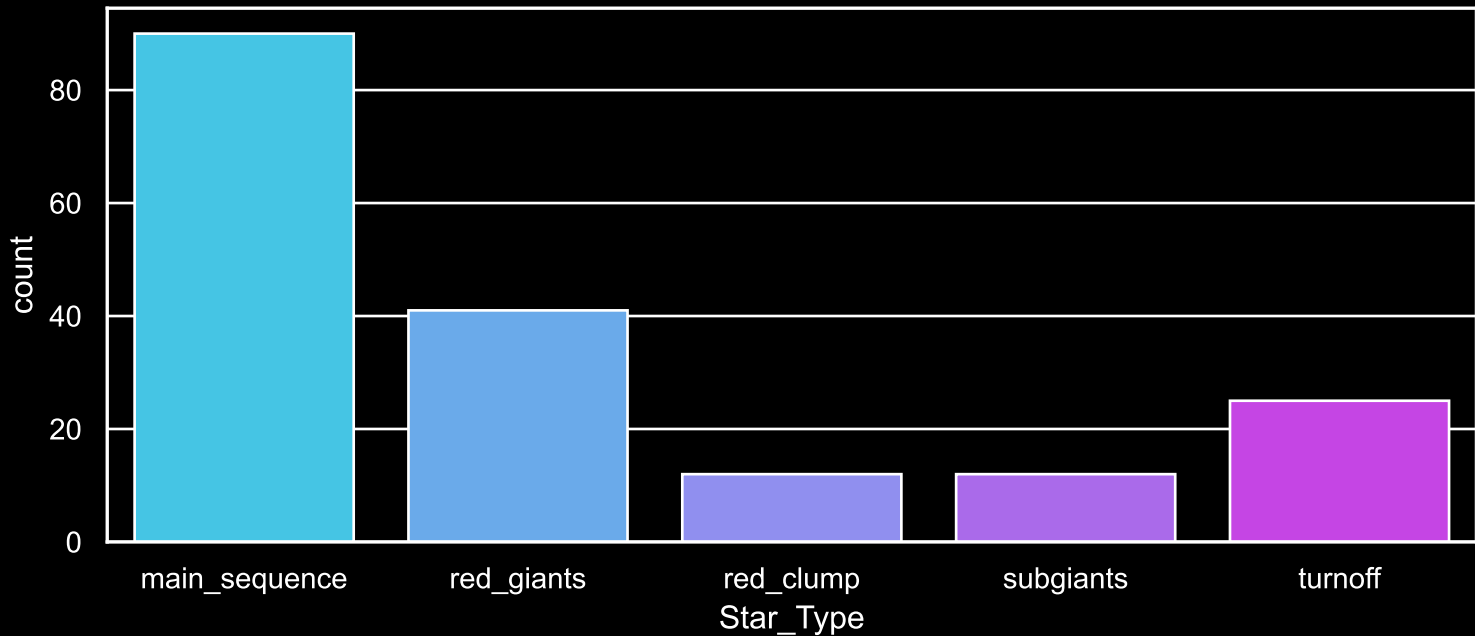
Field [43] Count plot of Star Type
