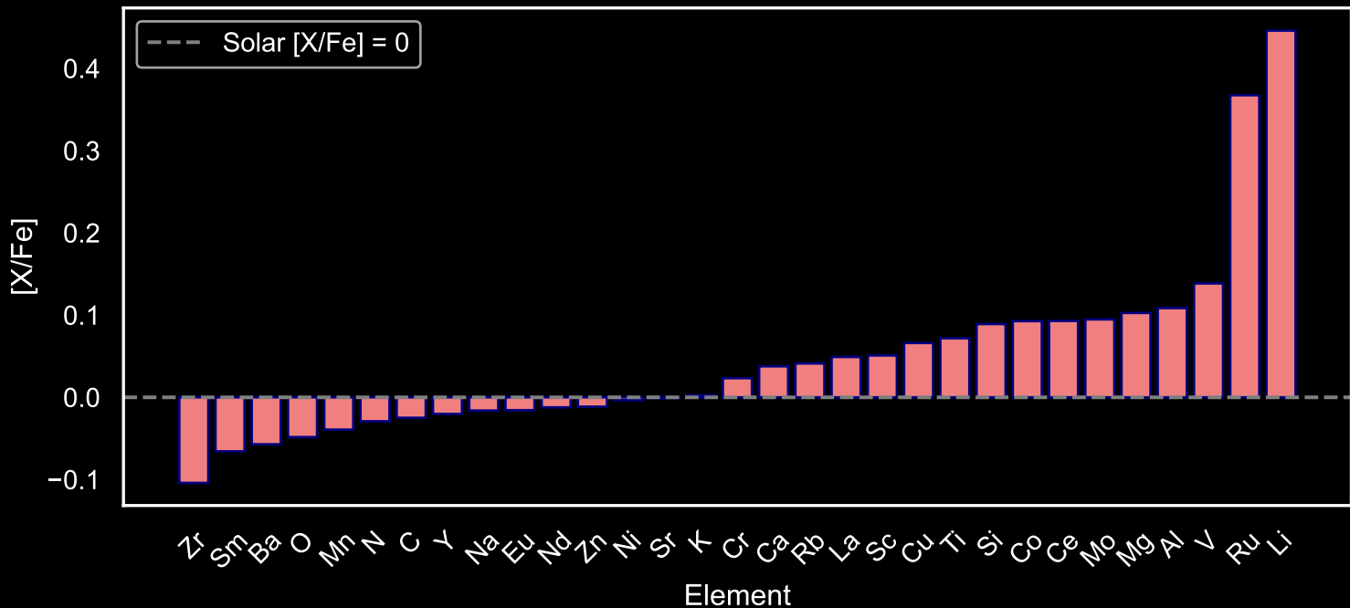
Abundance Pattern for GALAH Main Sequence Stars: Star Field [43] (N=90)
