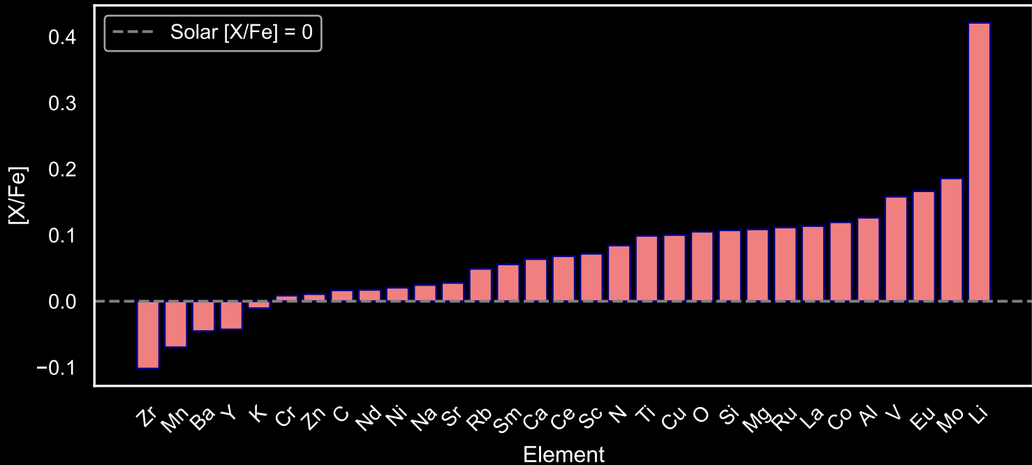
Abundance Pattern for GALAH Star Field [43] (N=180)
